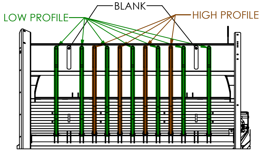
FACTORY HOOP LAYOUT
