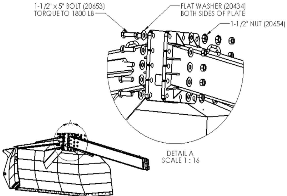
Figure 1 - Blade to hitch Attachment
