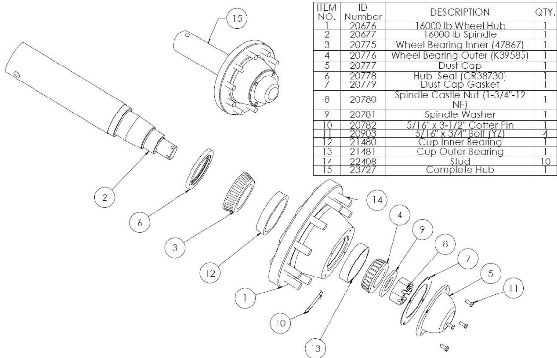
Figure 6 - Hub and spindle assembly
