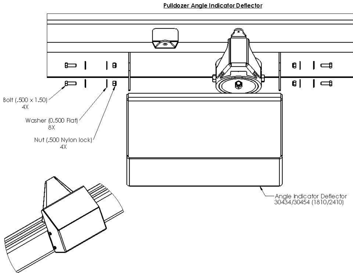
Figure 9 – Angle Indicator Deflector
