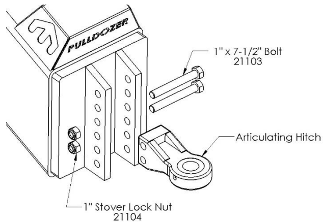
Figure 10 - Hitch installation (S/N PD1233 & Down)
